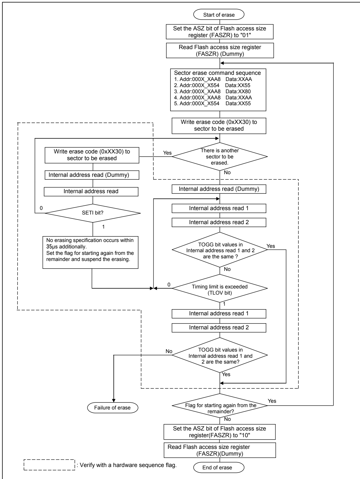
Figure 3-3 Example of sector erase procedure
