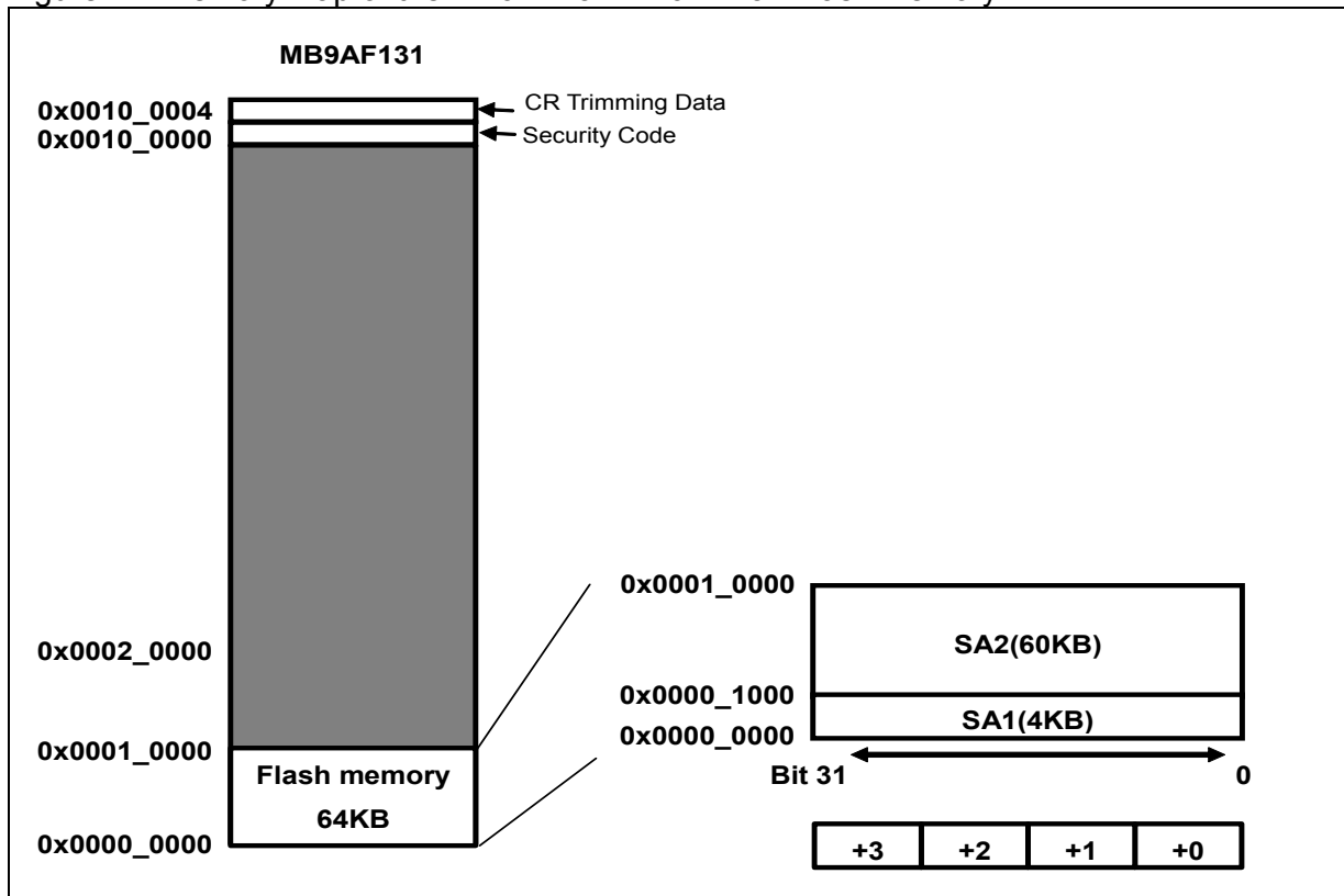
Figure 2-1 Memory Map of the MB9AF131/MB9AFA31 Flash Memory
