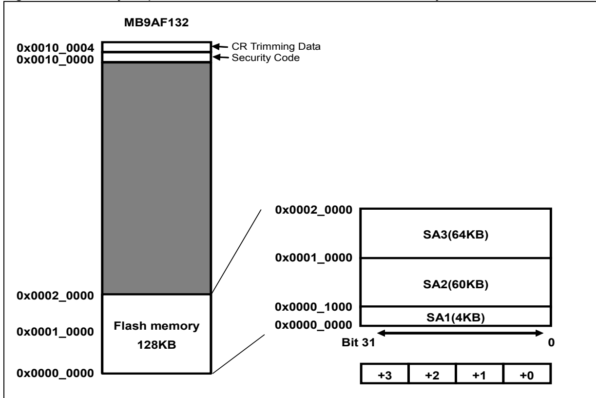
Figure 2-2 Memory Map of the MB9AF132/MB9AFA32 Flash Memory
