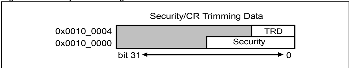
Figure 2-3 Security/CR Trimming Data Address
