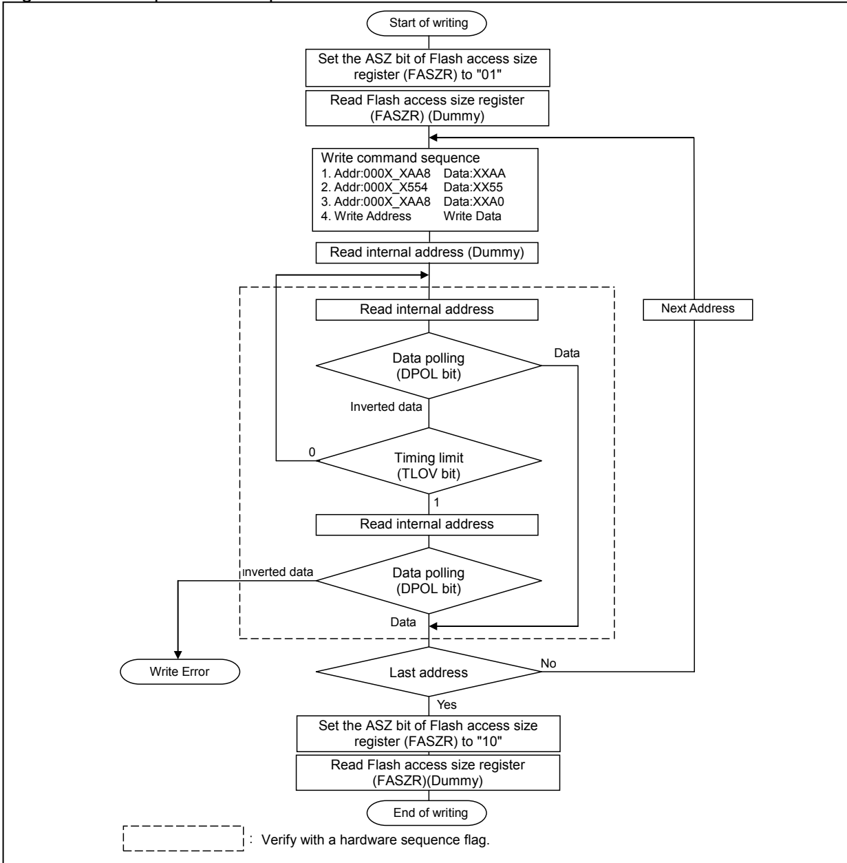
Figure 3-2 Example of write operation
